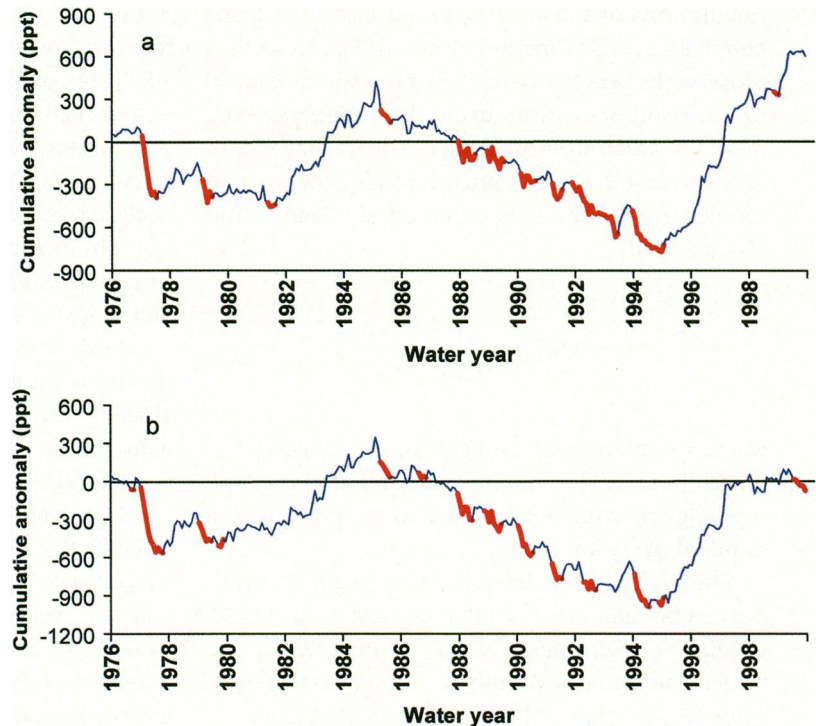
FIG. 3. Cumulative monthly precipitation anomalies for (a) Willamette Valley and (b) North Central Oregon climate divisions. Units are thousands (ppt) of annual mean precipitation. The final sum of anomalies is not zero because anomalies are computed with respect to long-term (105 yr) means for each month. Red segments indicate decile-identified drought periods.
