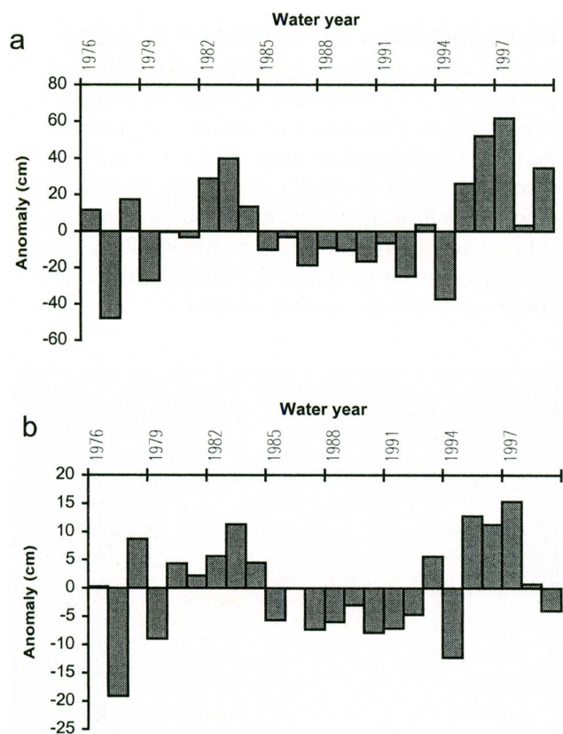
FIG. 2. Annual precipitation anomalies for (a) Willamette Valley and (b) North Central Oregon climate divisions. Long-term (105 yr) annual averages for the Willamette Valley and North Central divisions are 129 and 40.1 cm, respectively.
